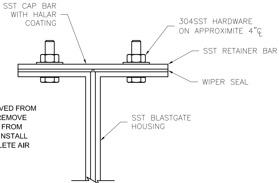
BLASTGATE DETAIL WITH GATES REMOVED IN OPEN POSITION
