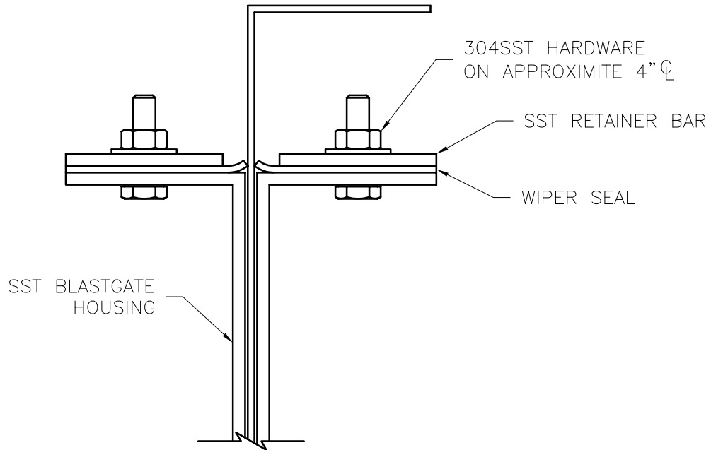
BLASTGATE DETAIL WITH GATES IN CLOSED POSITION
