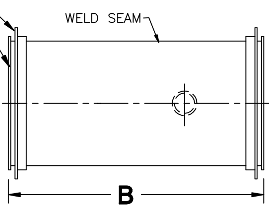
ELEV. VIEW
