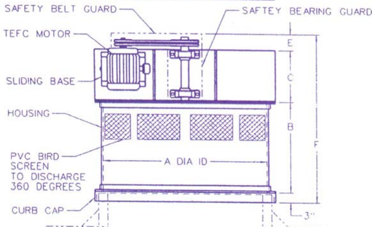
PRINCIPLE DIMENSIONS
